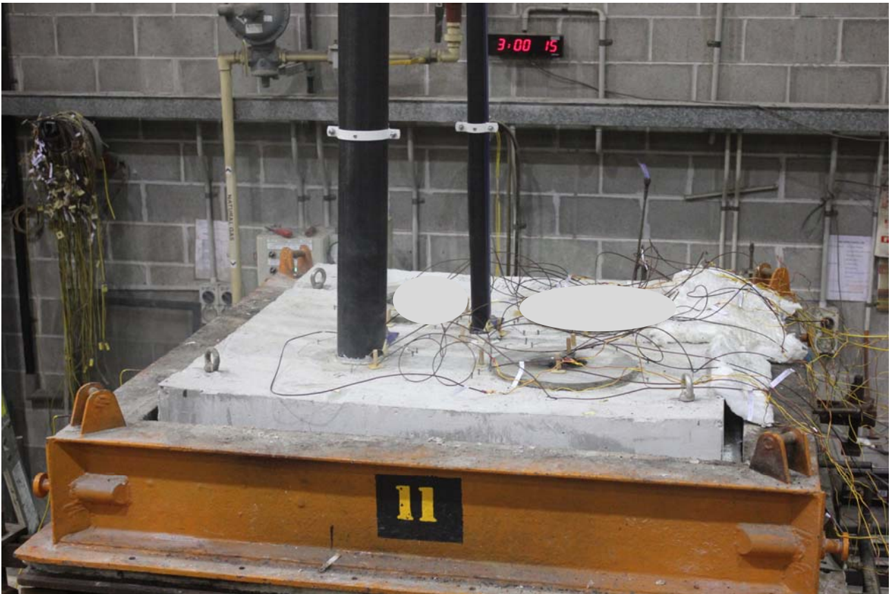
PHOTOGRAPH 9 – SPECIMENS AFTER 180 MINUTES OF TESTING
